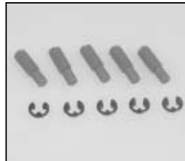
L4.74409.E threaded pins (5 pcs.) Gewindestifte (5 St.)
